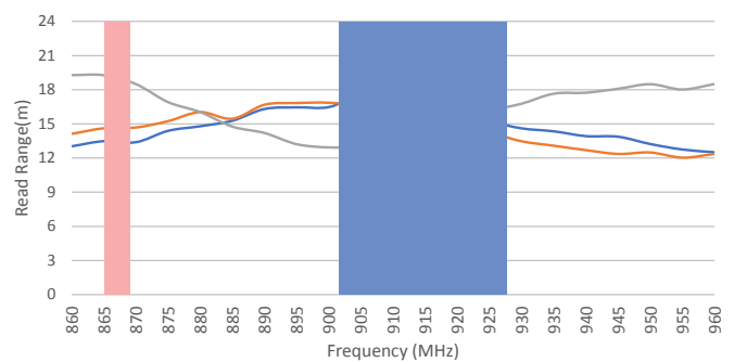
Read Range(2WERP)
