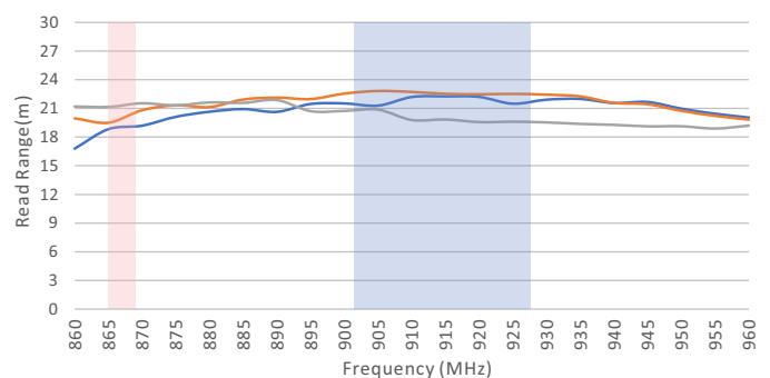
Read Range(2WERP)
